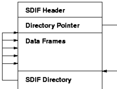
Figure 2 : Schema of an SDIF file with frame directory
