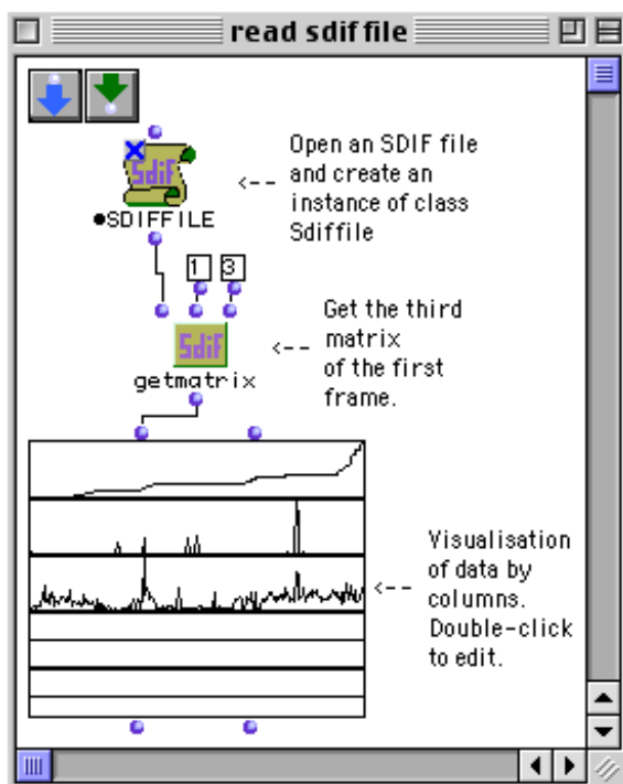
Figure 1: Reading from an SDIF file with OpenMusic
