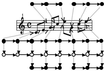
Fig. 5. First bar of Bach’s Prelude , a POC (below the score) associated to the 8-note PCC (white circles), and two POC for the 3-note PCC (over the score). These 3-note patterns are represented directly on the 8-note PCC with two additional POCs (at the bottom).
