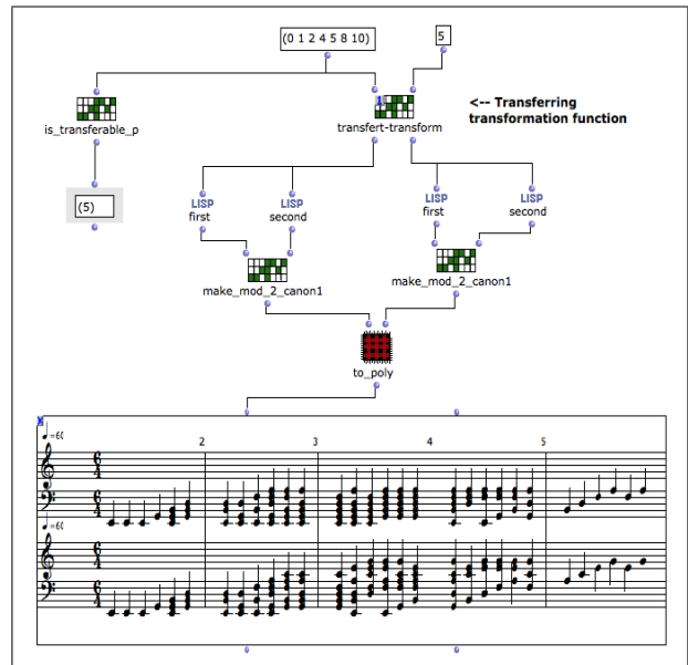
Figure 5. An OpenMusic patch returning two greater canons with the same donsets from a canon verifying the transferring condition.
