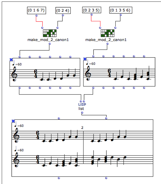
Figure 3. An OpenMusic patch representing two RT_2C of \mathbb{Z}_{12} . The upper one is not Vuza whilst the second one is.
