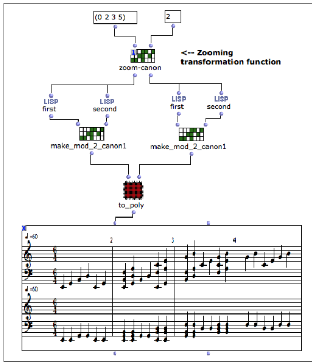
Figure 4. An OpenMusic patch returning two greater canons with the same donsets from a canon and a zooming coefficient, then representing them.
