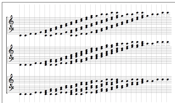
Figure 6. Three compact RT_2C of \mathbb{Z}_{30} with the same donsets.
