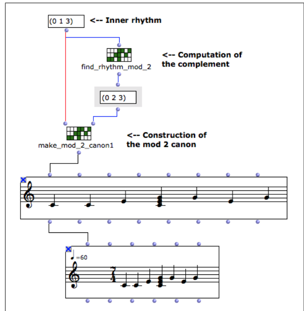
Figure 2. An OpenMusic patch, finding the outer rhythm forming a compact RT_2C , and representing it in traditional music notation.
