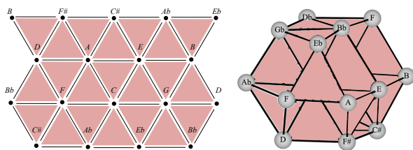
Figure 4. On the left, a region of the complex \mathcal{K}[3, 4, 5] composed by major and minor chords. On the right, the complex \mathcal{K}[2, 3, 3, 4] composed by dominant seventh and half-diminished chords.
