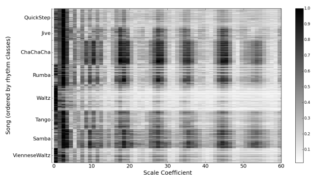
Figure 2: First 60 coefficients ( x -axis) of the Modulation Scale Spectrum for all the songs of the Ballroom test-set. The songs of the test-set are grouped by rhythm-classes on the y -axis. The coefficients are normalized : their amplitudes are represented in gray scale (black for a normalized amplitude of 1, white for 0)
