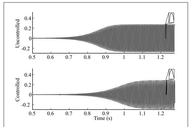
Figure 14. Attack transients of the self-sustained oscillating system with \gamma = 0.4 . Top: uncontrolled. Bottom: control applied with the aim of modifying the frequency of the second resonance, from f_2 = 448 Hz to f_2 = 470 Hz and reducing its damping by a factor of 2.
