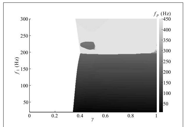
Figure 7. Map of the playing frequencies f_p (indicated by the depth of shading) of the notes played by the simulations plotted with respect to the frequency of the first resonance f_1 (ordinate) and to the pressure in the mouth of the musician \gamma (abscissa). White regions correspond to conditions under which no note is produced.
