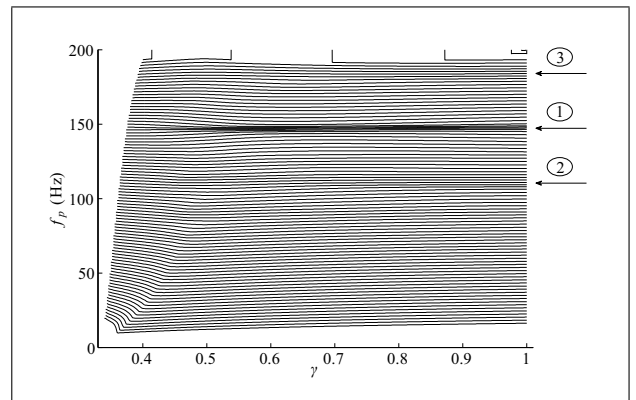
Figure 9. Playing frequencies f_p observed in the black region of Figure 7 ( 20 \text{ Hz} < f_1 < 196 \text{ Hz} ) plotted with respect to the mouth pressure \gamma . Each line stands for a single value of f_1 (i.e. a single target first resonance frequency). The first arrow indicates a region such that f_1 \approx f_2/3 , the second arrow indicates a region around f_1 \approx f_2/4 , and the third arrow indicates a region around f_1 \approx f_3/4 .
