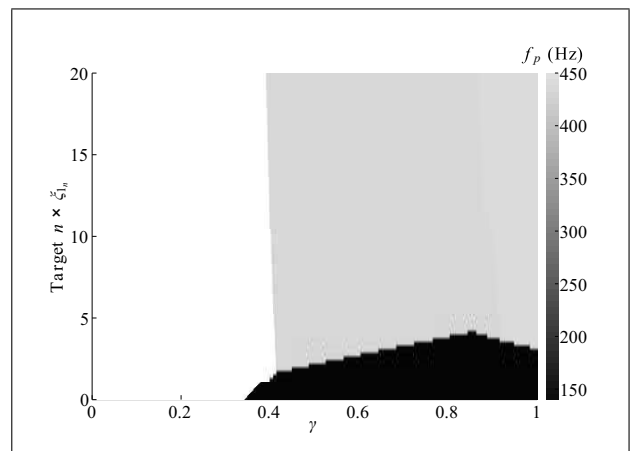
Figure 10. Map of the playing frequencies (indicated by the depth of shading) of the notes played by the simulations plotted with respect to the target modification of the damping of the first resonance (ordinate, \xi_1 = \text{value} \times \xi_{1_n} ) and to the pressure in the mouth of the musician \gamma (abscissa). White regions correspond to conditions under which no note is produced.
