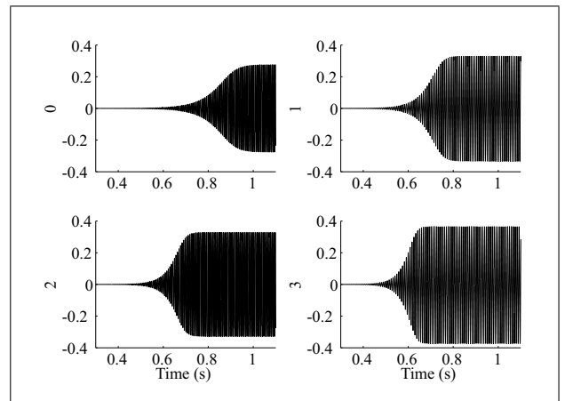
Figure 6. Attack transients of the self-sustained oscillating system with \gamma = 0.4 . Top left : Case 0 (uncontrolled). Top right : Case 1 ( f_1 = 120 Hz). Bottom left : Case 2 ( \xi_{1_n} reduced by a factor of 2). Bottom right : Case 3 ( f_1 = 120 Hz and \xi_{1_n} reduced by a factor of 2).
