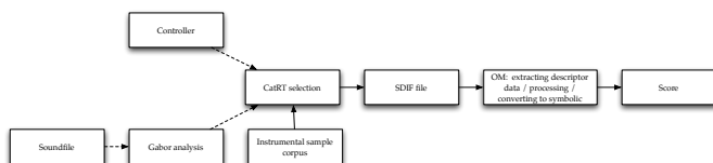
Figure 2. Flowchart for corpus-based transcription.
