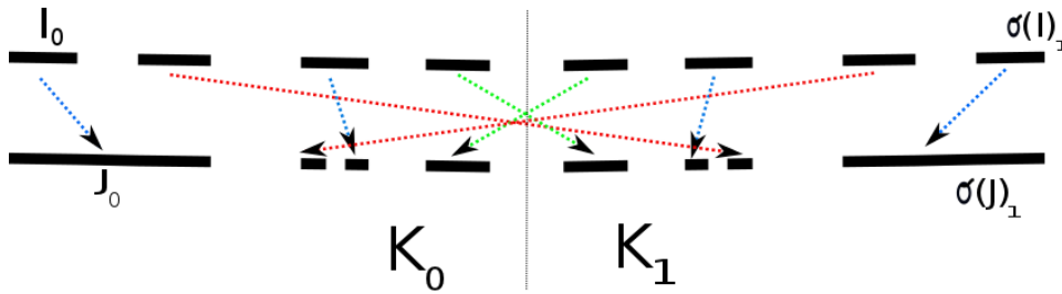
FIGURE 7. The corresponding element \phi(f) \in V_2 .
