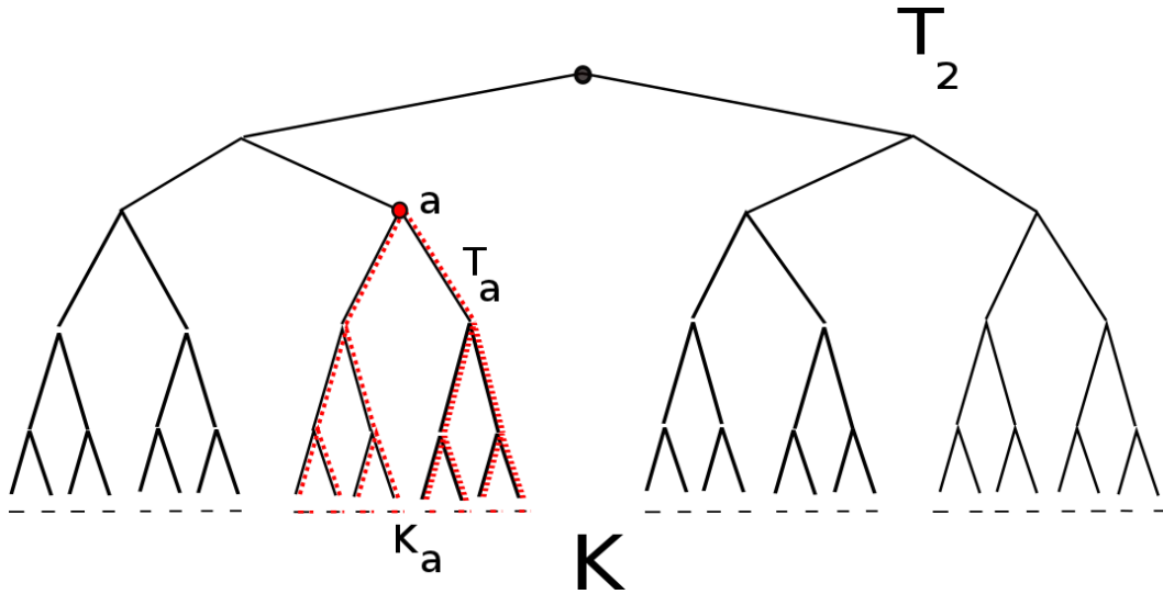
FIGURE 8. The rooted tree \mathcal{T}_2 , for a vertex a \in \mathcal{T}_2 , the tree \mathcal{T}_a and the elementary interval K_a are depicted
