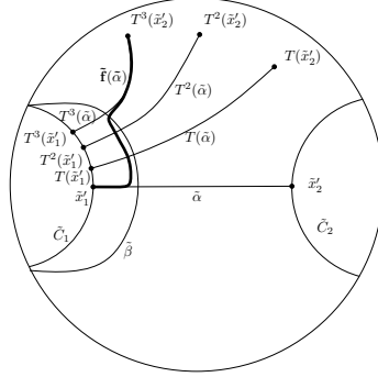
FIGURE 5. \tilde{f}^m(\tilde{\alpha}) in the case k = 3
