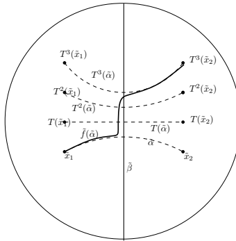
FIGURE 2. \tilde{f}(\tilde{\alpha}) in the case k = 3 (First subcase)
