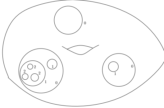
FIGURE 4. Level of curves of \mathcal{C}(f) .
