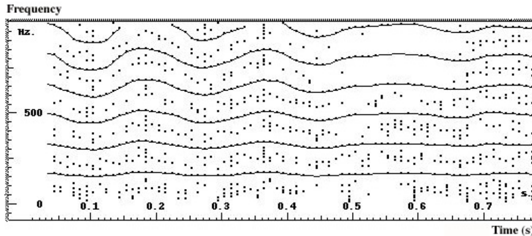
Fig. 1. Peaks found in successive analysis frames are grouped into tracks, i.e. sinusoidal partials.
