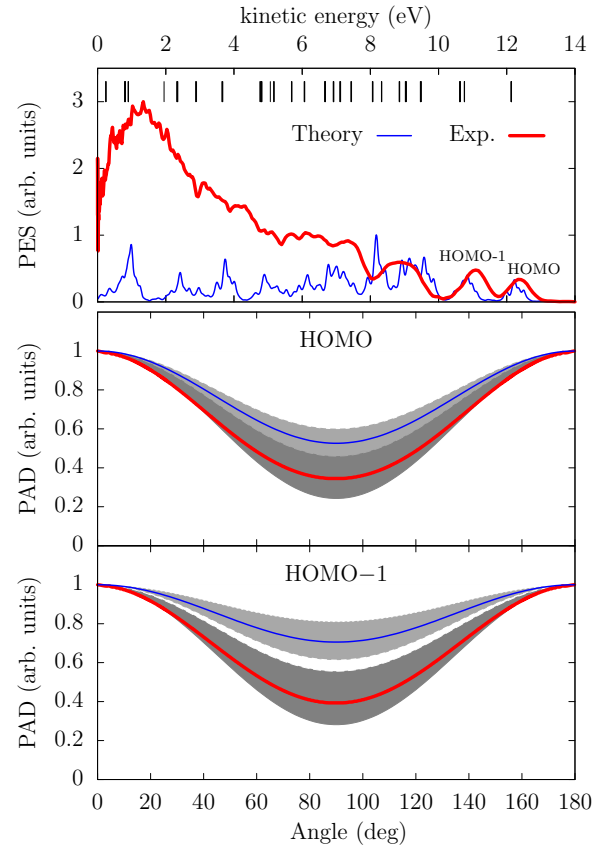
FIG. 2. (Color online) Top panel: Theoretical (blue thin line) and experimental (red thick line) photoelectron spectra under the conditions of Fig. 1 (one-photon regime). The vertical bars indicate the static single-particle density of states upshifted by the laser frequency and downshifted by 0.3 eV to account for the Coulomb shift due to a final ionization of 0.1. Middle and bottom panels: Corresponding angle-resolved distributions obtained from Legendre polynomial fits of the HOMO (middle panel) and HOMO-1 (bottom panel) levels. The shaded areas take into account the error bars in \beta_2 (0.25 for the experiment, in dark gray, and 0.1 for the theory, in light gray); see text for detail.
