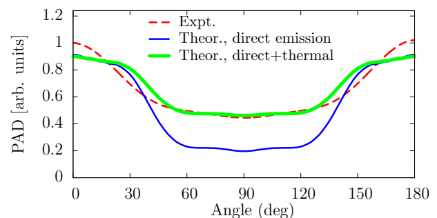
FIG. 4. (Color online) Experimental photoangular distribution from HOMO and HOMO-1 states (red dashed curve) of C_{60} in the same multiphoton regime as in Fig. 3, compared with total theoretical PADs, one taking into account only direct electronic emission (blue thin line) and the other one including in addition thermal fluctuations due to electronic temperature (green thick line).
