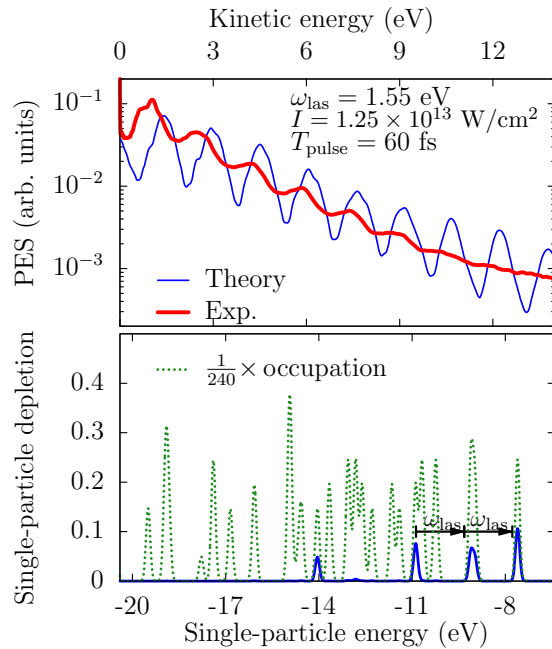
FIG. 3. (Color online) Multiphoton excitation of C_{60} with a laser of \omega_{\text{las}} = 1.55 eV, a duration of T_{\text{pulse}} = 60 fs, and an intensity of about 1.25 \times 10^{13} W/cm ^2 . Top panel: Comparison of theoretical (blue thin line) and experimental (red thick curve) photoelectron spectra in logarithmic scale. Bottom panel: Calculated depletions (blue solid) of single-particle states, compared with a density-of-states depletion from all orbitals (green dots). The single-particle energies have been downshifted by 0.2 eV to account for a Coulomb shift due to a total ionization of 0.06.
