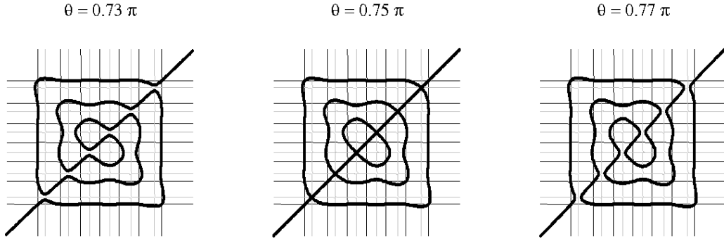
Figure 4: The nodal set of N(\Phi_n^\theta) near \frac{3\pi}{4} .
