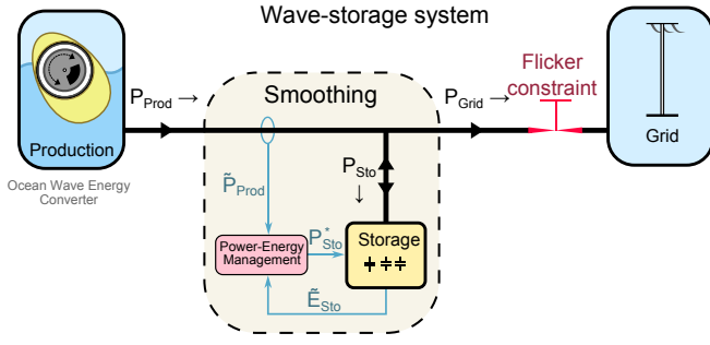
Fig. 9. Power smoothing with Energy Storage to satisfy a flicker constraint
