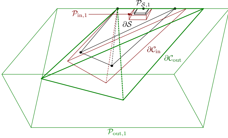
FIGURE 8. Prismatic neighborhoods of a 1-face in dimension 3
