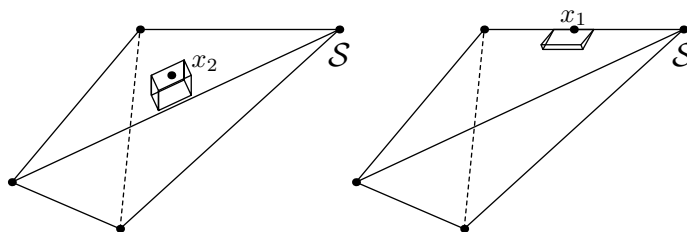
FIGURE 4. Prismatic neighborhoods of a point in a 1-face and a 2-face in dimension 3
