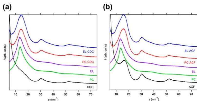
Figure 2. XRD patterns of carbon, PC-impregnated carbon (PC-carbon), and \text{Et}_4\text{NBF}_4 -PC-impregnated carbon (EL-carbon): CDC (a) and ACF (b).
