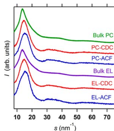
Figure 3. Corrected XRD patterns of PC and \text{Et}_4\text{NBF}_4 -PC confined in pores of CDC and ACF and the XRD pattern of bulk PC at 303 K.
