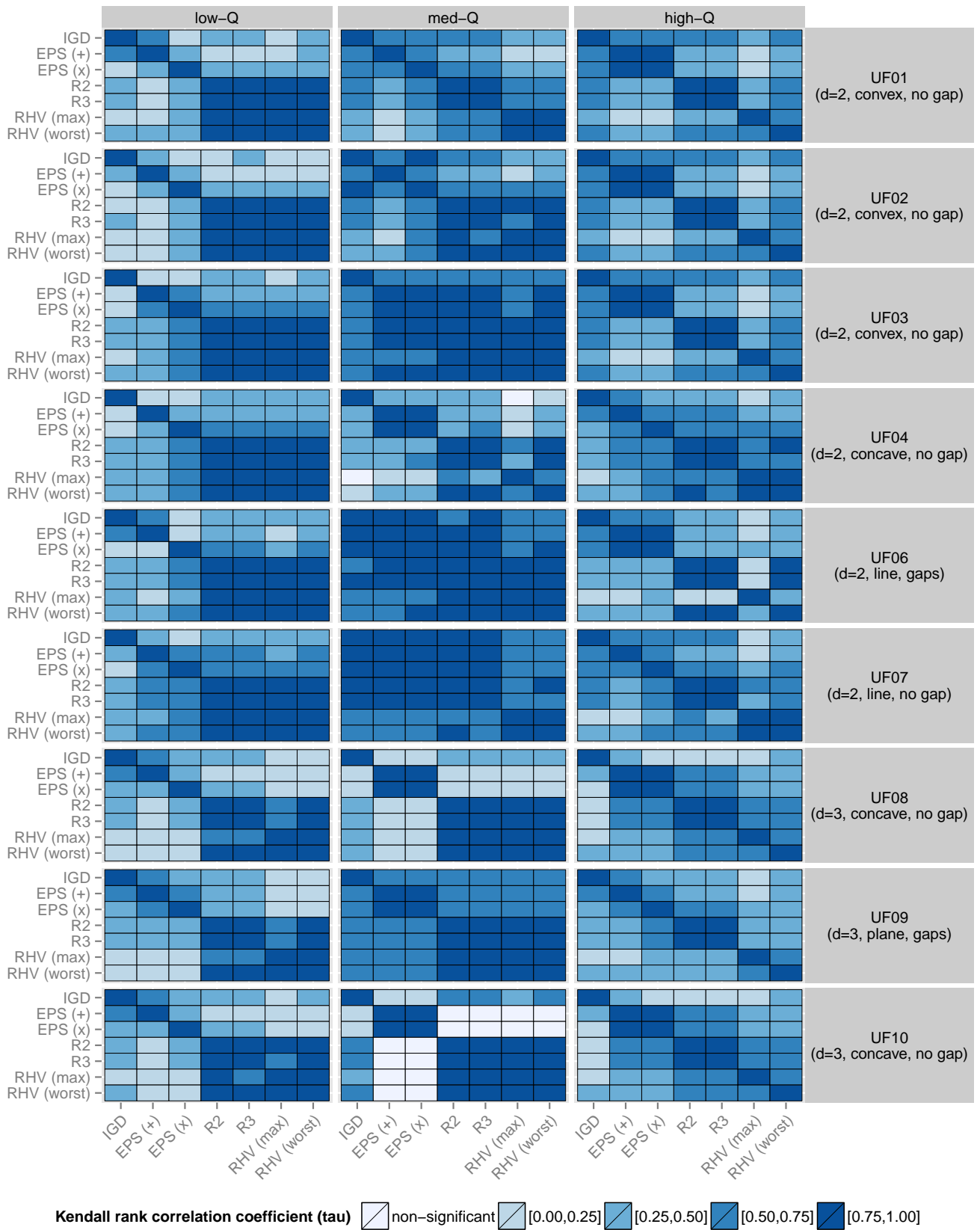
Figure 1: Heat-map Kendall rank correlation \tau for each pair of set quality indicators (displayed on both axes), each sampling strategy (low-Q, med-Q, high-Q) and each problem function (UF01–UF10).
