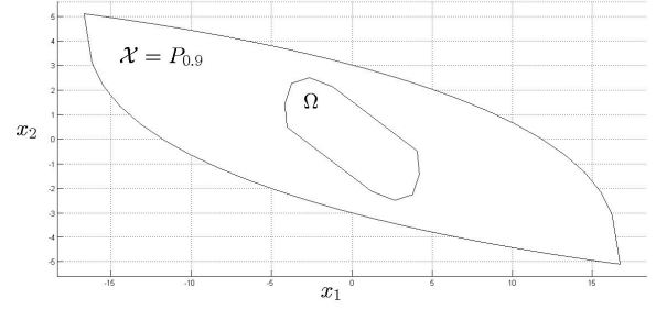
Fig. 1. The maximal disturbance invariant set \Omega and domain of attraction \mathcal{X} = P_{0.9} .
