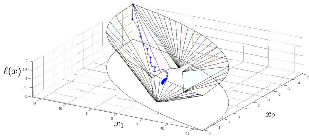
Fig. 5. The strict decrease of \ell(x) over \mathcal{X} \setminus \Omega along the state.
