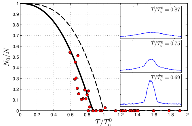
FIG. 4. (Color online). Condensate fraction across the BEC transition as a function of temperature. The experimental data (red points) is compared to the theory for an ideal Bose gas (dashed black line) and to the theory including mean-field interaction in the BEC component (solid black line) [42]. Data is plotted only for T/T_c^0 > 0.6 as fitting bi-modal distributions becomes unreliable at low temperatures. Inset: 1D Density profiles of the gas taken after time-of-flight and at various temperatures across the BEC transition.
