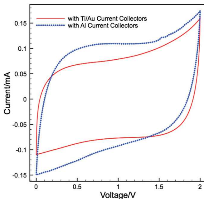
Fig. 7. CV curves at 100 \text{ mV s}^{-1} for devices with different types of current collectors in 1 \text{ M NEt}_4\text{BF}_4 in PC.
