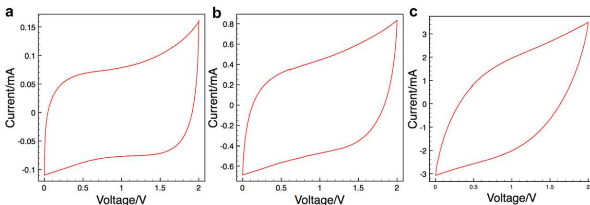
Fig. 6. CV curves of the micro-supercapacitor at scan rates of a) 100 \text{ mV s}^{-1} , b) 1 \text{ V s}^{-1} and c) 10 \text{ V s}^{-1} with Ti/Au current collectors in 1 \text{ M NEt}_4\text{BF}_4 in PC.
