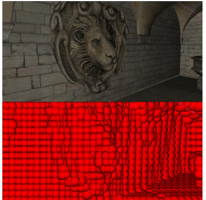
Figure 10. This image exposes the bounding spheres of each geometry cluster. These spheres are used to quickly reject group of view samples that are not affected by a cone.
