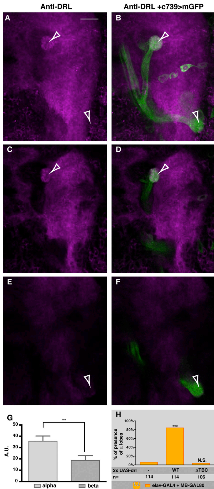
Figure 5. DRL Is Present at the Tips of the MB Lobes, and DRL's TBC Site Is Required to Rescue the Mutant Phenotype
