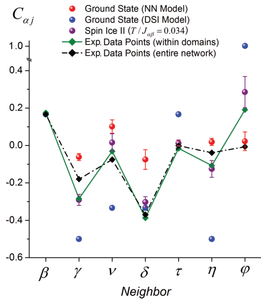
FIG. 2. (Color online) Average values of the pairwise spin correlators defined up to the seventh neighbor and computed within the charge domains (green diamonds, full line) and at the network scale (black diamonds, dashed line). For comparison, values expected for the ground-state manifolds of the nearest-neighbor (NN) SI model and DSI model are represented as red and blue spheres, respectively. The purple spheres correspond to the values given by Monte Carlo simulations for a temperature of T/J_{\alpha\beta} \simeq 0.034 , which best fits the experimental data. The error bars represent the numerical standard deviations of each correlation type at a given temperature and are computed over the set of sampling Monte Carlo snapshots (see note [33]). The lines linking the experimental data points have no physical meaning and are just guides for the eyes.
