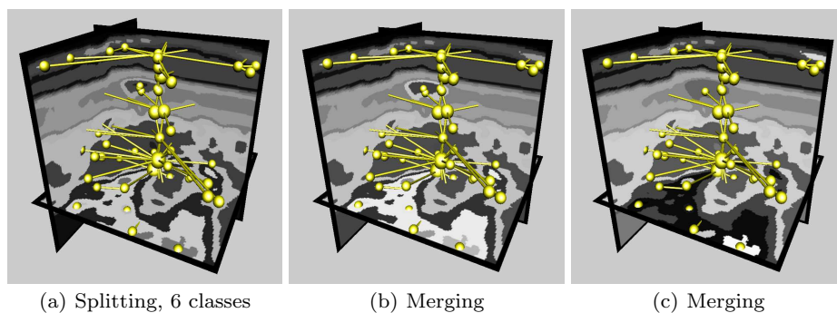
Fig. 13: Scenario 2: Figure 11(a) is segmented using three operations: one splitting operation and two merging operations. Vertices represent regions that have been identified during the segmentation process and an edge links two vertices if their corresponding regions are adjacent. The users perform merging and splitting operations by clicking on specific vertices or edges in the graph (see sub-section 6.1 for more details).
