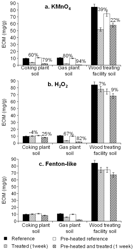
Figure 1: Extractable organic matter (EOM) content for the references (one week in water) and samples treated with (a) KMnO 4 , (b) H 2 O 2 and (c) Fenton-like (one week), with/without pre-heating (±SD; percentages correspond to the EOM decrease rate after the treatments compared to the reference counterparts)
