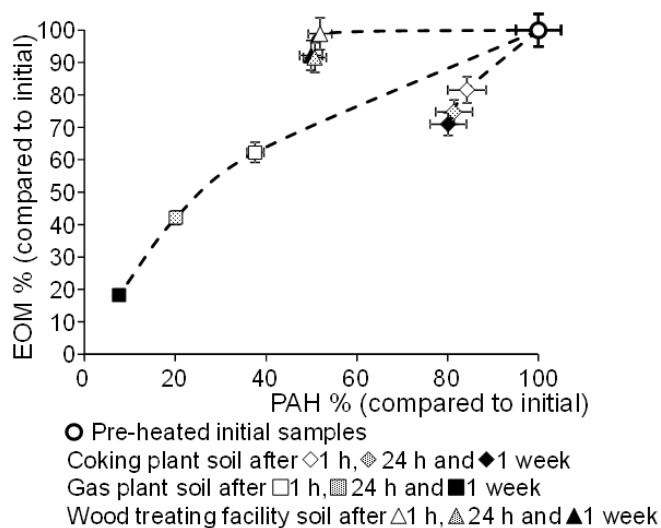
Figure 3: Extractable organic matter (EOM) and PAH proportions related to the initial samples 1, 24 h and one week after H 2 O 2 application in the pre-heated soils ( \pm SD)
