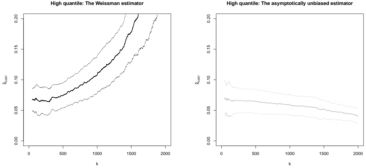
(a) The Weissman estimator
