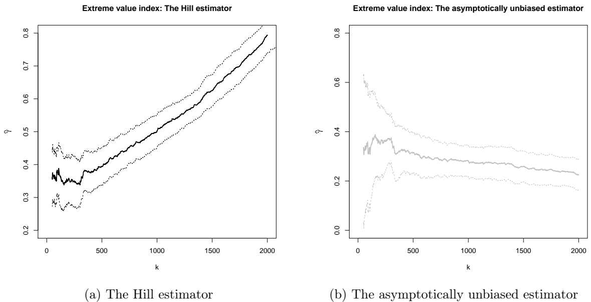
Figure 11: Estimating the extreme value index for the DJIA index. The figures present the estimates of the extreme value index for the loss returns of the DJIA index with varying choice of k . The left panel uses the Hill estimator. The right panel uses the asymptotically unbiased estimators of the extreme value index in Section 4.2. The confidence interval is obtained from the block bootstrapping method.
