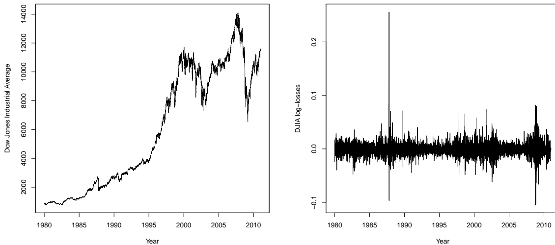
(a) Dow Jones Industrial Average (DJIA).
