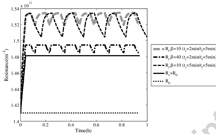
Figure 13: Relaxation effect on membrane fouling ( t_r : filtration time, t_e : relaxation time)
