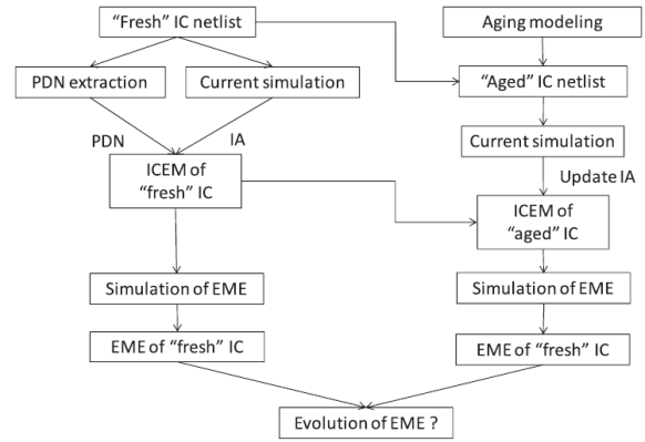
Figure 5: Aging-aware ICEM construction flow [2].
