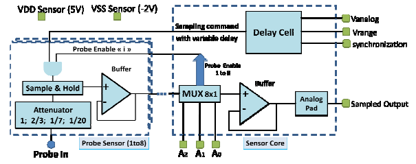
Fig. 2 Sensor-on chip architecture
