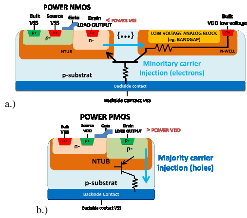
Fig. 1 Wafer cross section of power a.)NMOS b.)PMOS
