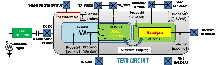
Fig. 6 Description of the conducted EMI test
