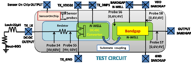
Fig. 4 Coupling between power and low voltage analog blocks
