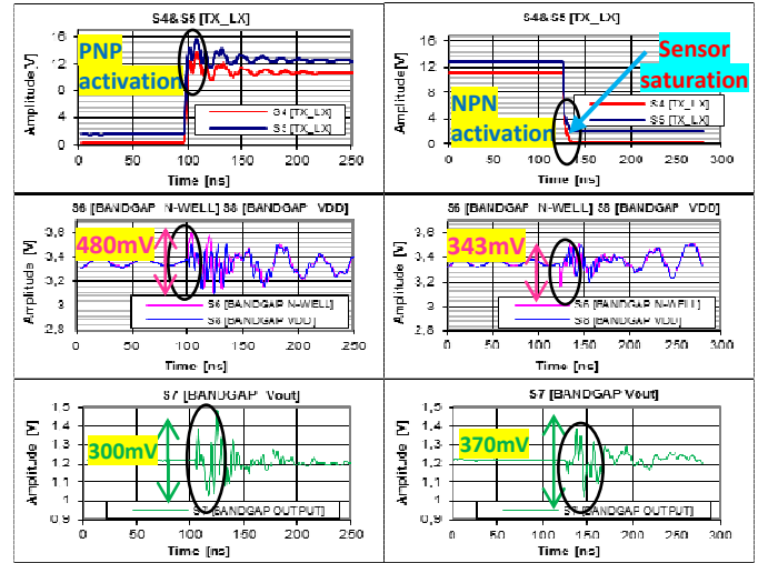
Fig. 5 DC-DC output effects on Bandgap power supply and output (left colon: rising edge; right colon: falling edge)
