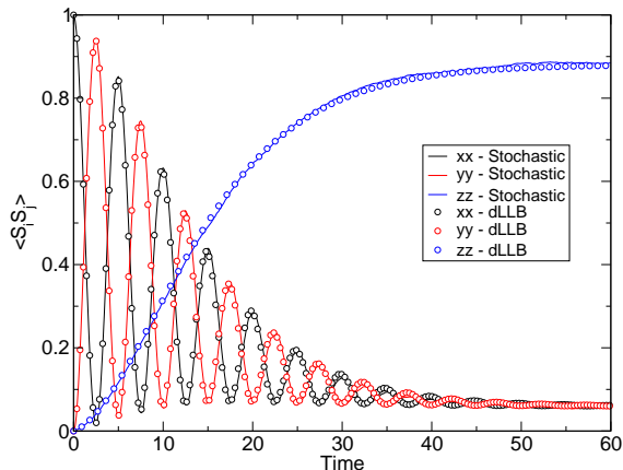
Figure 2: Relaxation of the diagonal components of the correlation tensor \langle s_i s_j \rangle . Again, the solid lines plot the stochastic case (1000 averaged repetitions) and the dots are for the dLLB model. Initial conditions: \langle s_1(0)^2 \rangle = 1 , and \langle s_i(0) s_j(0) \rangle = 0 \forall (i, j) \neq (1, 1) .
