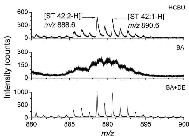
Figure 6. Part of the TOF-SIMS negative ion mass spectra recorded at the surface of a rat cerebellum section, using HCBU, BA, and BA+DE setting modes and showing sulfatide ion peaks.
