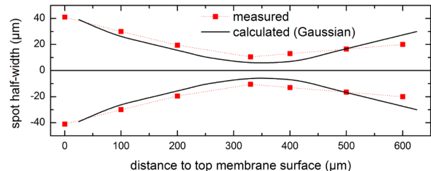
Figure 12: Measurement of VCSEL spot width as a function of the axial position (red squares, dotted line) and comparison with calculated beam profile assuming Gaussian beam propagation (black line).
