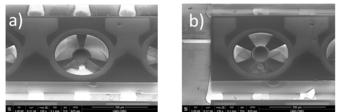
Figure 6: Top-view SEM image after lens micro-spotter deposition on a treated surface using a) DMSE (contact angle= 32^\circ ) b) polyester (contact angle= 46^\circ ).
