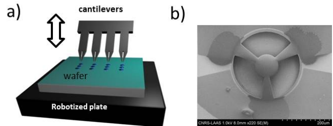
Figure 5: a) Principle of lens deposition using a robotized silicon-cantilever micro-spotter. b) SEM image of membrane surface after deposition of DMSE without surface treatment.
