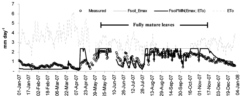
Figure 2 Comparison of measured daily tree transpiration (Measured; opened circle) and estimated daily E_{Tree} of F_{soil}E_{max} model (thin line) and F_{soil} * MIN(E_{max}; ET_0) model (bold line). The gray dotted line indicates the daily ET_0 .
