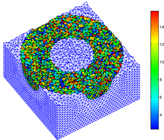
Figure 1: Realization of the random field \{C_{11}(\mathbf{x}), \mathbf{x} \in \Omega_{int}\} (in GPa) in the interphase region (meshed view of the continuum model).
