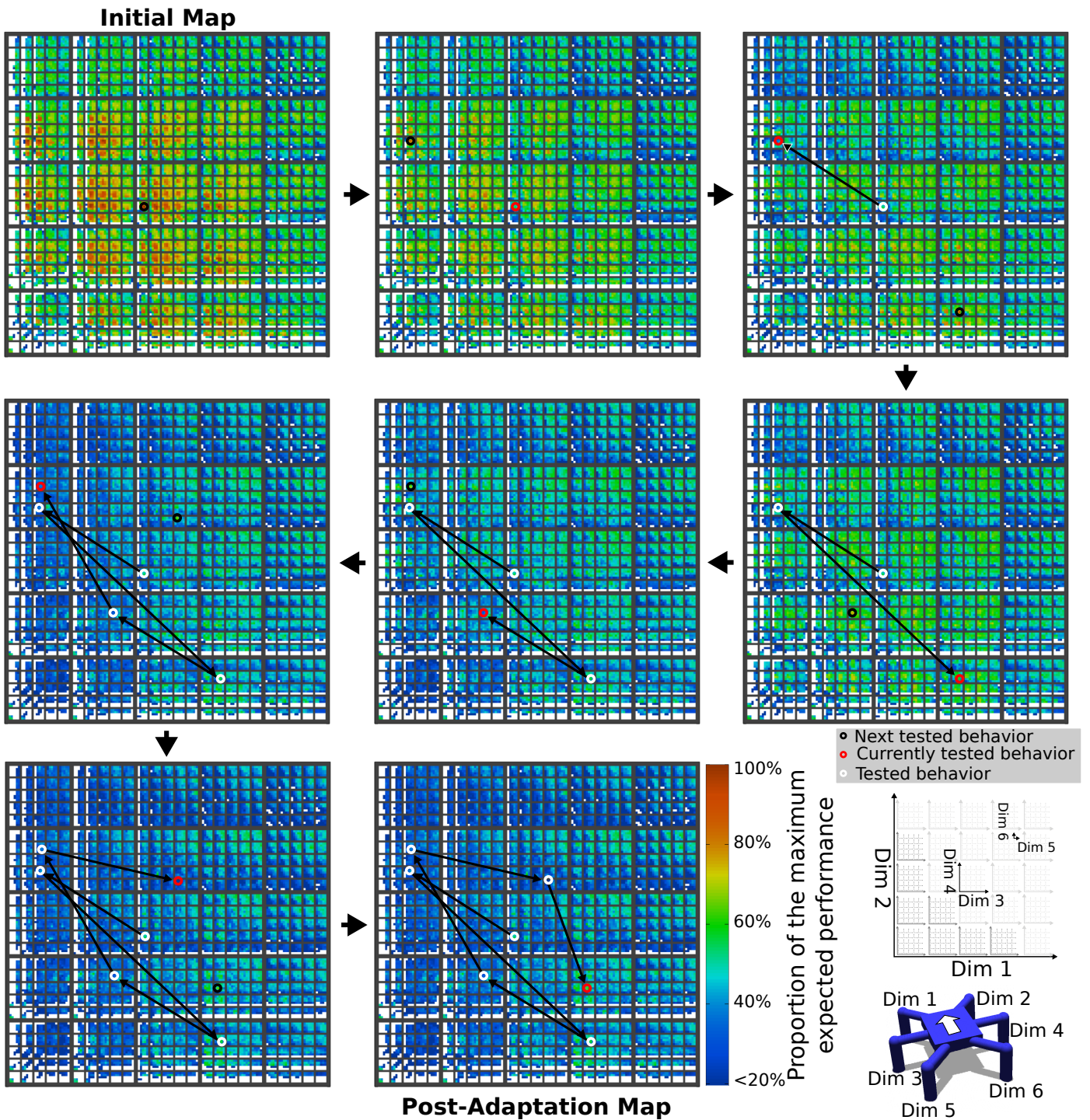
Extended Data Figure 6 | How the behavior performance map is explored to discover a compensatory behavior (non-normalized to highlight that performance predictions decrease as it is discovered that predictions from the simulated, undamaged robot do not work well on the damaged robot). Colors represent the performance prediction for each point in the map relative to the highest performing prediction in the first map. A black circle indicates the next behavior to be tested on the physical robot. A red circle indicates the behavior that was just tested (note that the performance predictions surrounding it have changed versus the previous panel). Arrows reveal the order that points have been explored. The red circle in the last map in the sequence is the final, selected, compensatory behavior. In this scenario, the robot loses leg number 3. The six dimensional space is visualized according to the inset legend. The data visualized in this figure are identical to those in the previous figure: the difference is simply whether the data are renormalized for each new map in the sequence.
