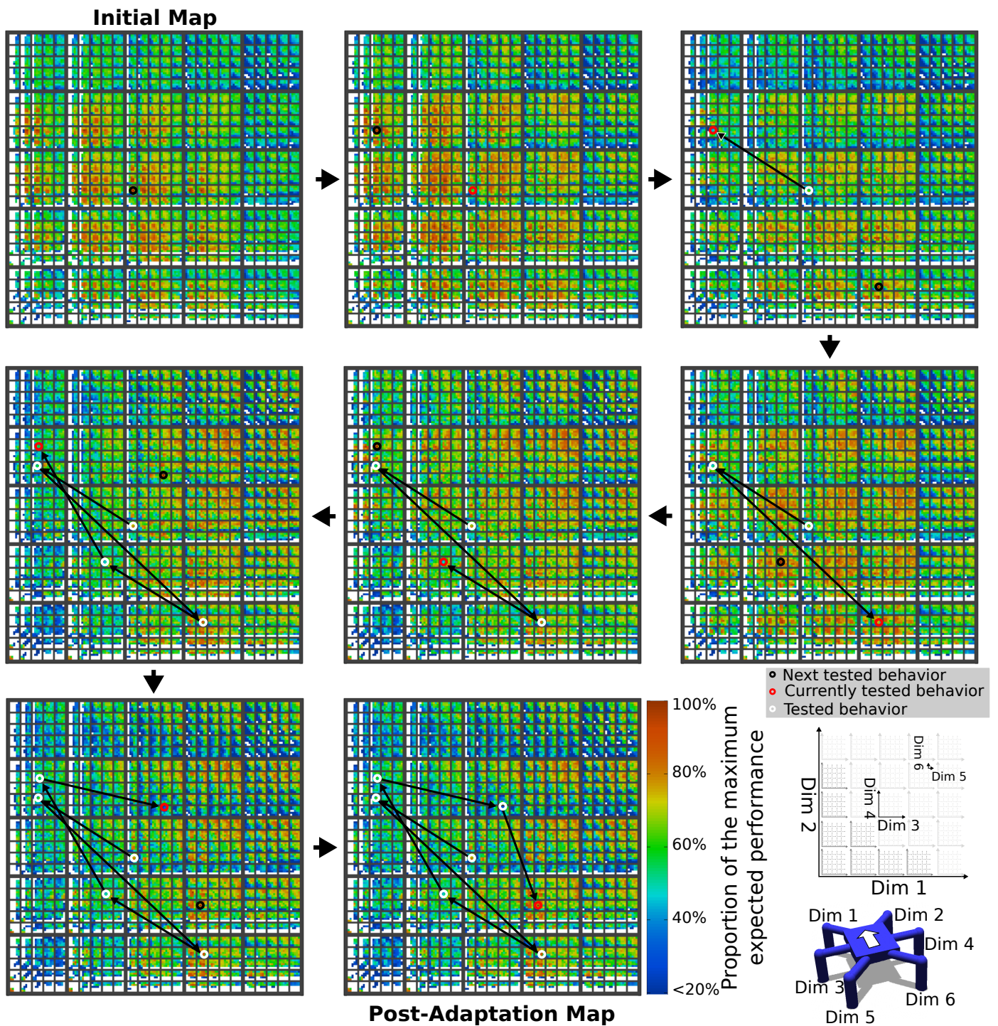
Extended Data Figure 5 | How the behavior performance map is explored to discover a compensatory behavior (normalized each iteration to highlight the range of remaining performance predictions). Colors represent the performance prediction for each point in the map relative to the highest performing prediction in the map at that step of the process. A black circle indicates the next behavior to be tested on the physical robot. A red circle indicates the behavior that was just tested (note that the performance predictions surrounding it have changed versus the previous panel). Arrows reveal the order that points have been explored. The red circle in the last map is the final, selected, compensatory behavior. In this scenario, the robot loses leg number 3. The six dimensional space is visualized according to the inset legend.
