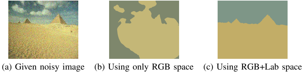
Fig. 1. Segmentation results for a noisy image (a) without the dimension lifting in Stage 2 (b) and with Stage 2 (c).
