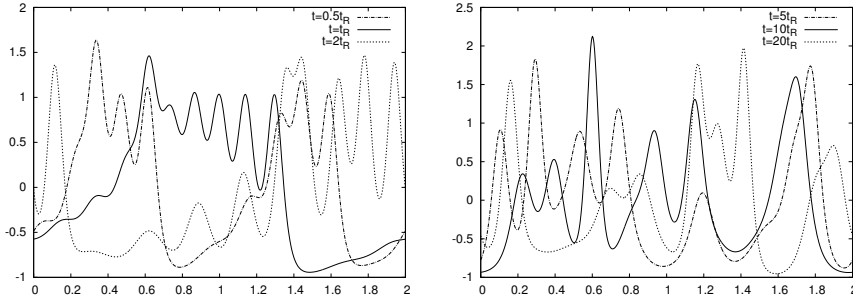
Fig. 8 Test-case 3: Numerical solution at times t = 0.5t_R , t_R , 2t_R , 5t_R , 10t_R and 20t_R . Computation done with K = 160 elements, a polynomial degree N = 5 and a time step \tau = 2.5 \cdot 10^{-4} .
