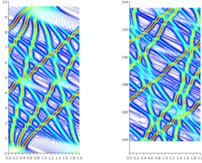
Fig. 10 Test-case 3: Contour levels of the numerical solution in the (x, t) -plane, between times 0 and t_R at left, between times 19t_R and 20t_R at right. Computation done with K = 160 elements, a polynomial degree N = 5 and a time step \tau = 2.5 \cdot 10^{-4} .
