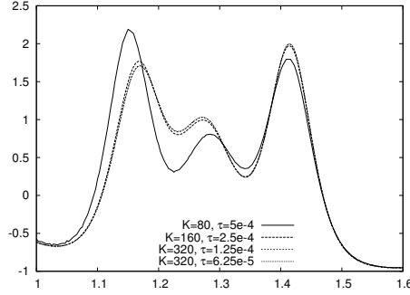
Fig. 9 Test-case 3: Zoom of the numerical solutions at times 20t_R . Computations done for various values of the number of elements K and time-step \tau , and with a polynomial degree N = 5 .
