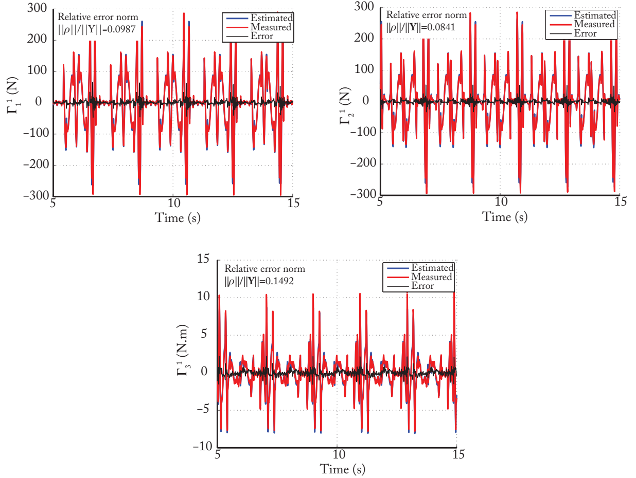
Figure 5: Values of \mathbf{\Gamma}^1 , estimated from input torques using the relation \mathbf{J}_p^{inv T} \boldsymbol{\tau} from (30) (red lines) and calculated using identified parameters \hat{\boldsymbol{\chi}} from the relation \mathbf{IDM}\boldsymbol{\chi} (blue lines) with the payload of 5.37 kg.
