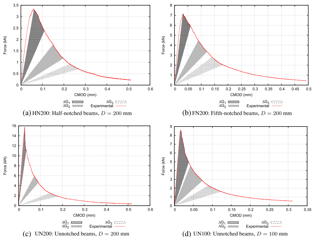
Figure 11. Different intervals of dissipated energy represented on the averaged force versus crack mouth opening displacement (CMOD) experimental curves.
