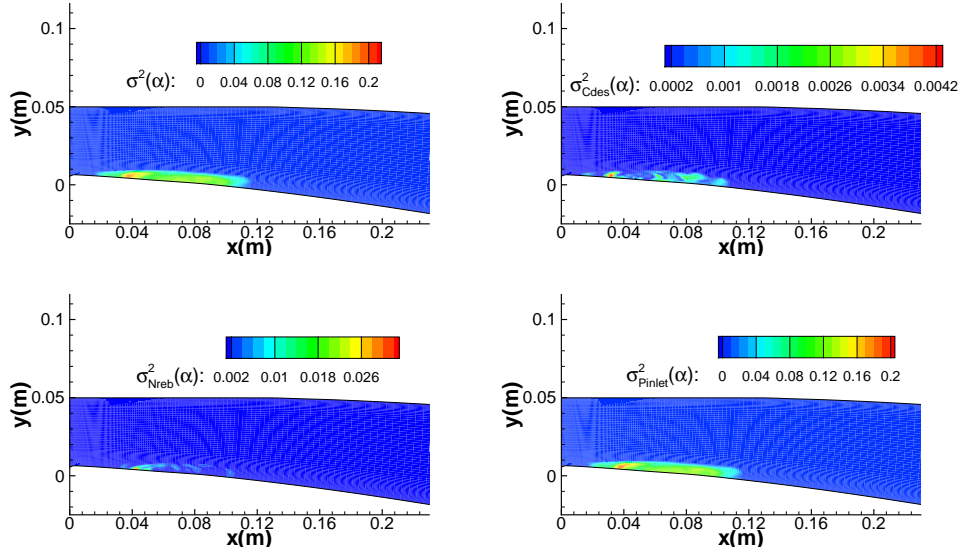
Figure 5: Sensitivity indices of the void ration at a time t = 1.5 s.
