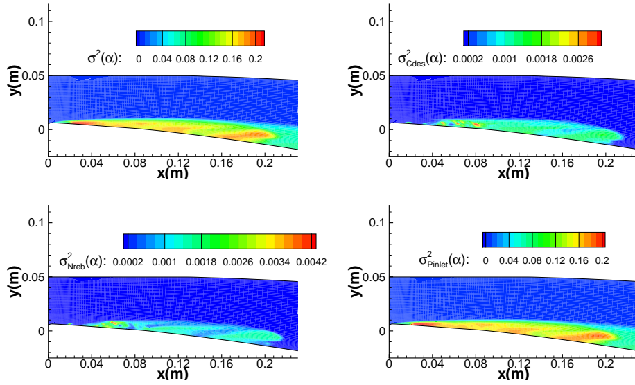
Figure 6: Sensitivity indices of the void ration at a time t = 2.28 s.
