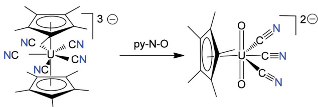
Scheme 9 Synthesis of the uranyl cyanide [\text{UO}_2(\text{Cp}^*)(\text{CN})_3]^{2-} .
