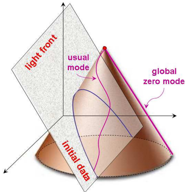
Figure 1: The past light cone of an event in spacetime. All world-lines intersect the light front hypersurface in a finite time, except the one parallel to it. The latter corresponds to the global zero mode.
