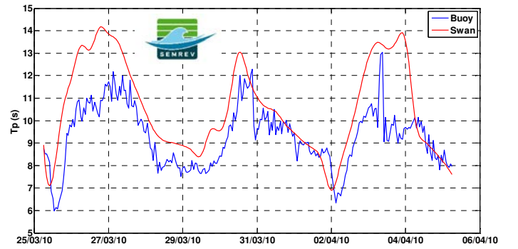
Figure 7: Comparison between buoy measurements and Swan model estimates ( T_{p,R5} ) during the event number 3.
