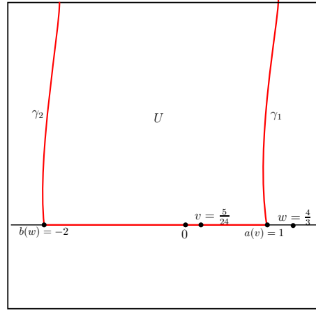
Figure 5. Bijective region of f = \frac{1}{2}z^2 - \frac{1}{6}z^3 - \frac{1}{8}z^4
