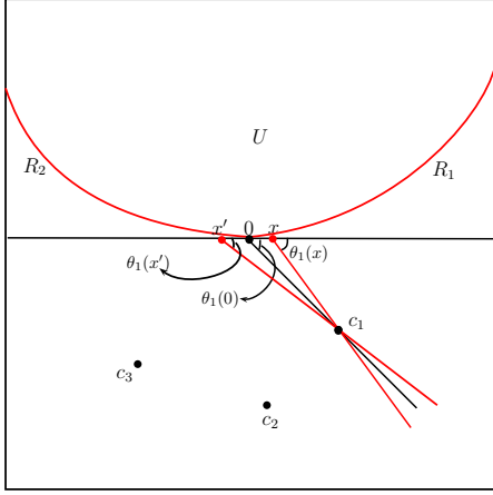
Figure 4. The same sign of \theta_1(0) - \theta_1(x) and x
