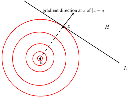
Figure 2. Gradient direction of z \mapsto |z - a|
