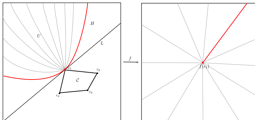
Figure 1. Bijective region of f
