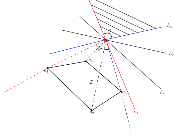
Figure 3. The intersection of all H_j
