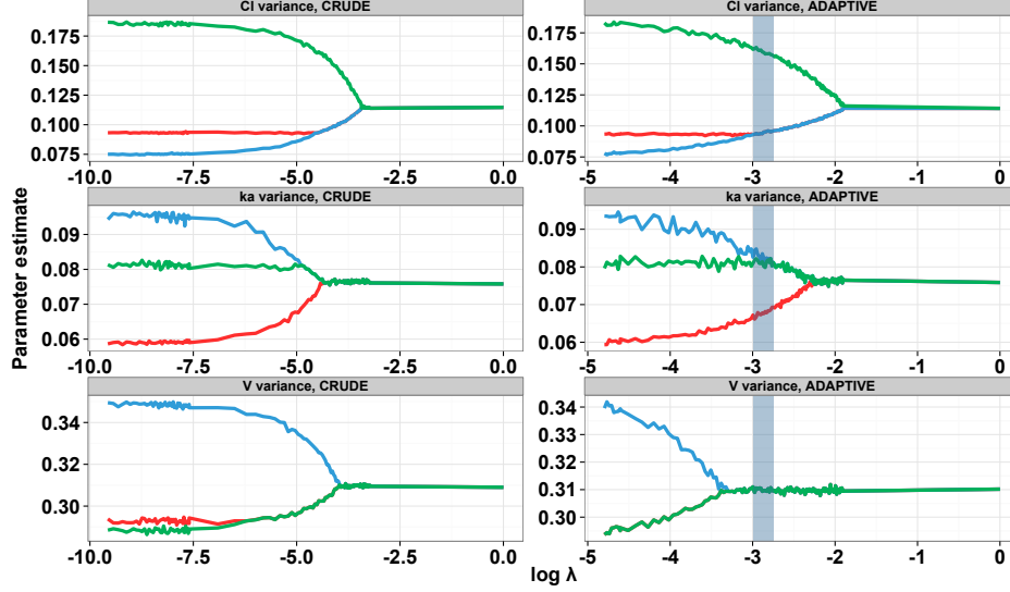
Figure 4: Simulated data, 3 groups, large \omega_V , small \omega_{k_a} : regularisation paths of SAEM estimates for random effect variances with (ADAPTIVE) or without (CRUDE) adaptive weights. Red, blue and green curves correspond respectively to the estimates in group 1, 2 and 3. Blue shaded areas correspond to the values \Lambda that return the simulated differences model.
