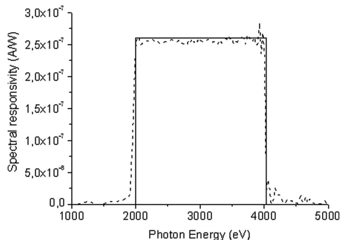
FIG. 14. Ideal spectral responsivity of the channel (solid line) and calculated total responsivity (dashed line).
