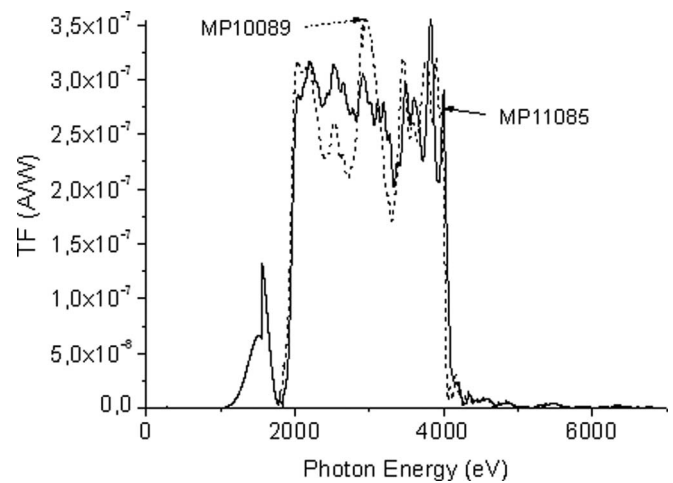
FIG. 6. Spectral responsivity of the MLM channel for two different mirrors.
