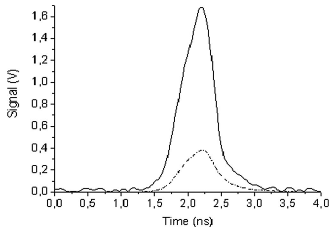
FIG. 9. Signal measured with the MPI1085 MLM channel, designed for the spectral range from 2 keV to 4 keV, and signal part due to the remaining reflectance at lower photon energies (dashed).
