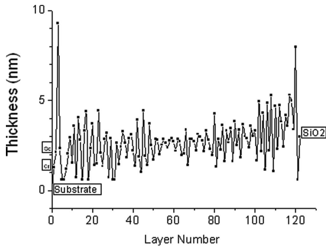
FIG. 11. Layer thicknesses for the optimized MLM designed for a grazing angle of 1.9^\circ . The Cr layers are odd-numbered; the Sc layers are even-numbered.
