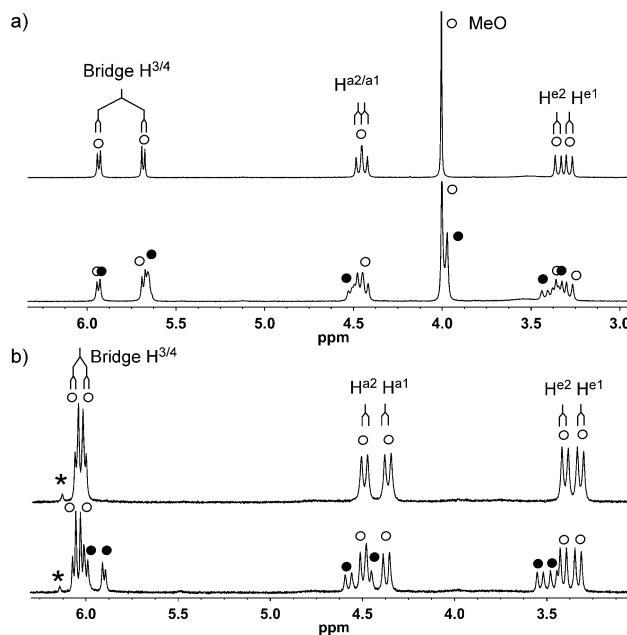
Fig. 1 Selected portions of room temperature 1 H spectra before (top) and after (bottom) saturation of the solvent with xenon. (a) (MeO) 3 -111 in CDCl 3 , (b) Br 3 -111 in nitrobenzene- d 5 . Open and filled circles represent signals of the free and xenon-occupied hosts, respectively. *Represents the homodimeric hexabromo derivative ( Br 6 -111 ), found as an impurity (~2%).
