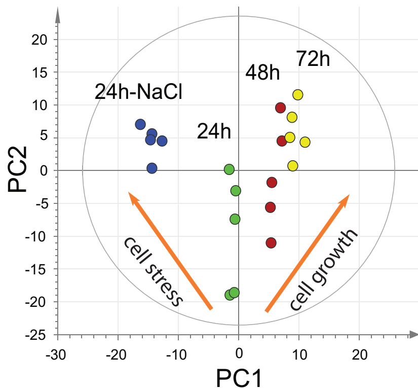
Figure S1. PCA score and its corresponding loading plot of all ^1\text{H} HR-MACS data acquired for the two studies, cell stress and cell growth. ( R^2X(\text{cum}) = 0.793 ; Q^2(\text{cum}) = 0.737 ).
