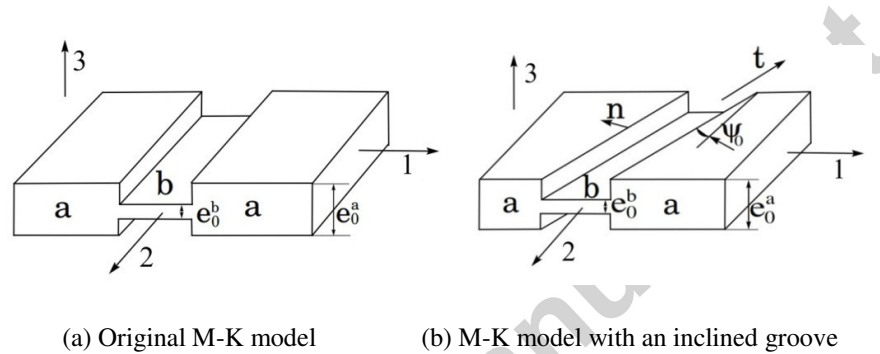
Fig. 1. Representation of the M-K model.
