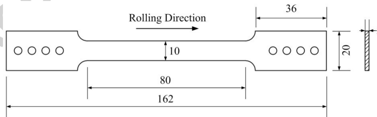
Fig. 2. Geometry and dimensions of the tensile specimen (unit: mm).
