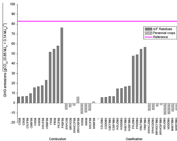
Fig. 4. Greenhouse gas (GHG) emissions of bioenergy (i.e. bioheat and bioelectricity) compared to fossil fuel based combined heat and power (CHP) systems. The bars represent the total emissions of each bioenergy production pathway whereas the solid line above the bars represents the GHG emissions of the fossil fuel based CHP system.
