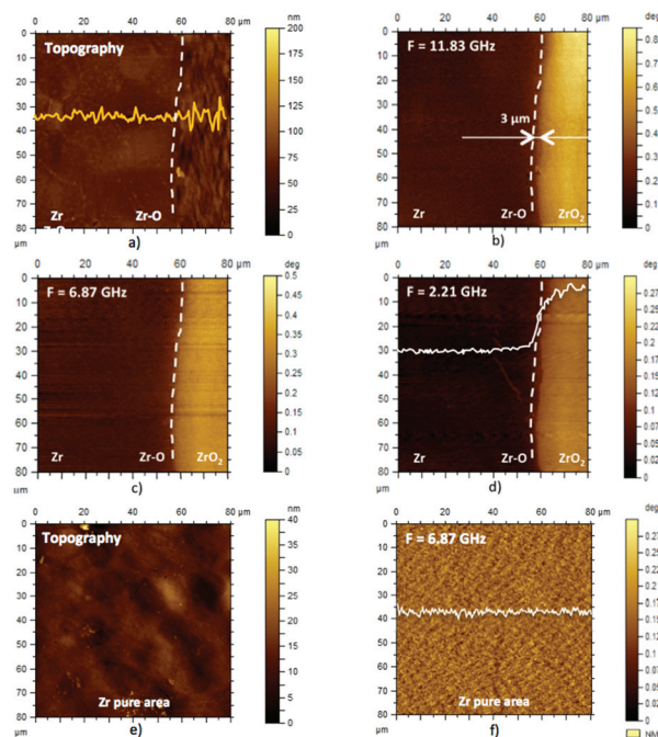
Fig. 4 Topography and phase shift cartography for several frequencies (scan area 80 \mu\text{m} ). (a) Topographical image of the sample and a cross-section. (b) Phase shift image at f = 11.83 GHz. (c) Phase shift image at f = 6.87 GHz. (d) Phase shift image at f = 2.21 GHz. (e) Topographical image of pure Zr. (f) Phase shift image of pure Zr at f = 6.87 GHz.
