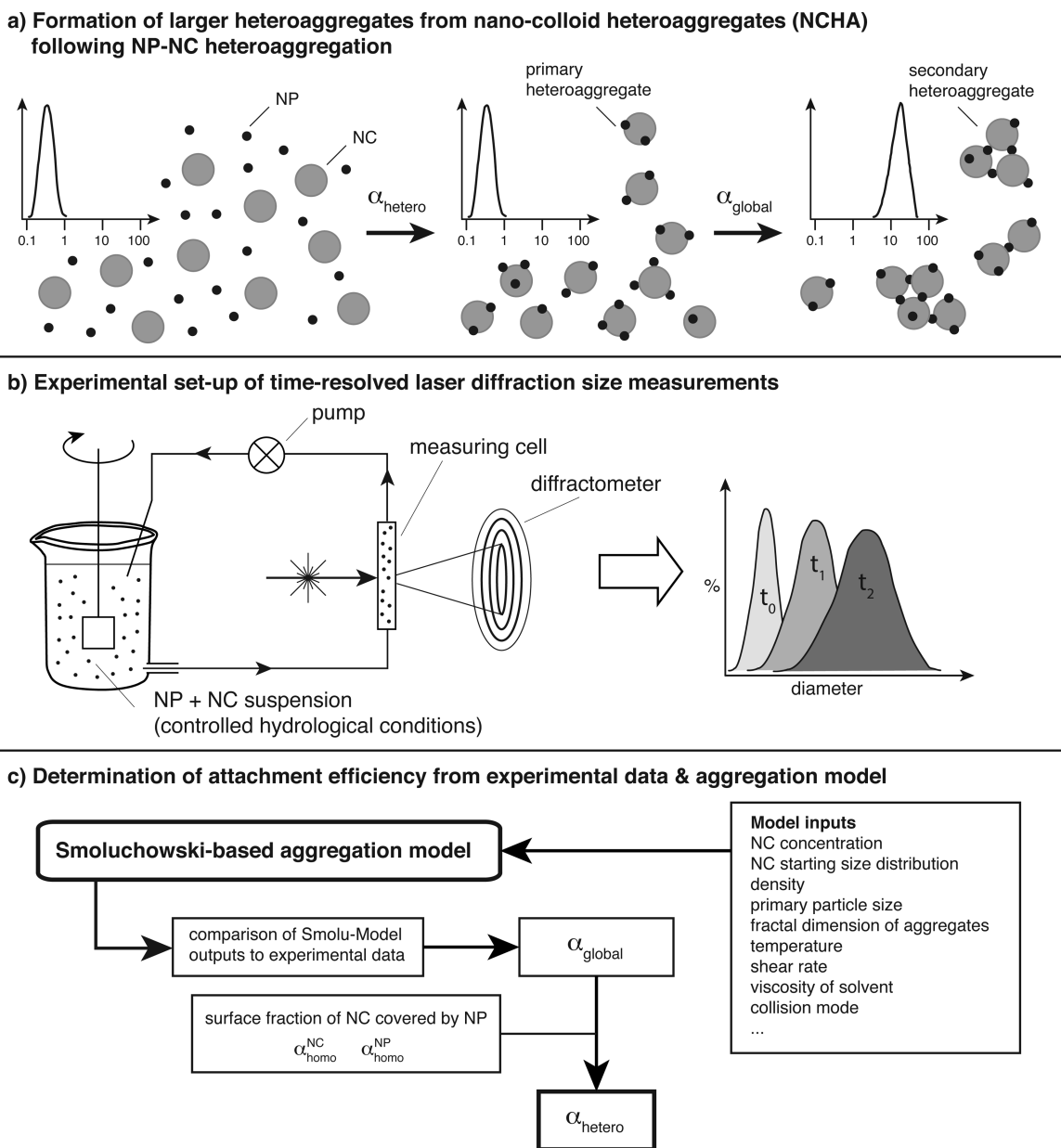
Figure 1. Overview of the general concept developed in this study to determine attachment efficiencies for heteroaggregation, \alpha_{hetero} . (a) The aggregation of small NPs with larger NCs, first forming NP-NC primary heteroaggregates which then further aggregate with each other to form larger secondary heteroaggregates. (b) Experimental setup. (c) The data interpretation with an aggregation model and calculation of \alpha_{hetero} is visualized.
